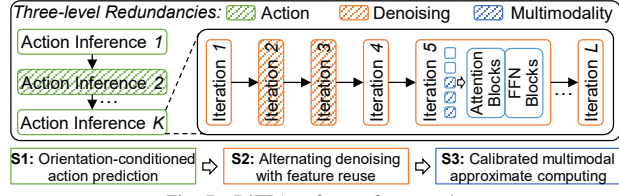
Fig. 7. DiTPA software framework.
