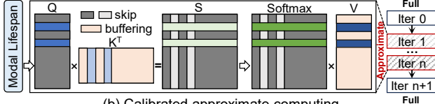
Fig. 9. Calibrated approximation for vision and language modality.
