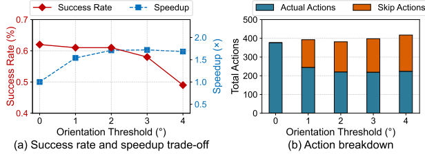
Fig. 21. Trajectory accuracy and performance evaluation.
