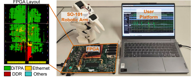
Fig. 25. Deployment on Lerobot SO-101 robotic arm.
