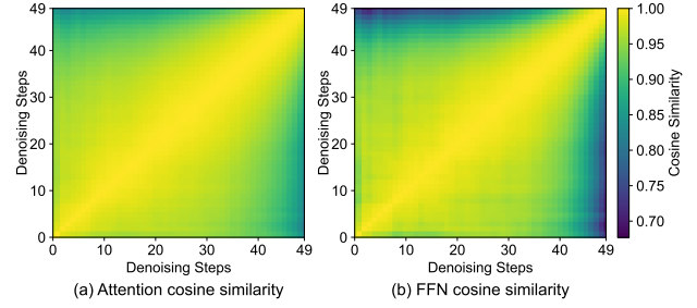
Fig. 5. Denoising redundancy analysis.
